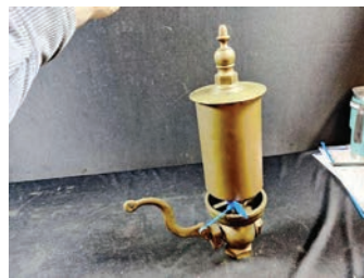
Lot # 7275 Great 4" Brass Chime whistle
