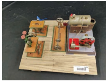
Lot # 6470 Weeder Model steam engine shop set up running model nice set
