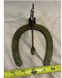
Lot # 4732 BLACKSMITH'S HORSESHOE GAUGE
