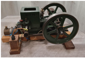
4767 Model 1/2 Horse Witte hit miss engine working model sweet little engine
