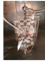
136 Finish Pump / Kremlin Spray gun, 15 years old works good
